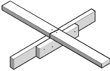
(a) Butt-joint with block fixed to side of rafter/truss
