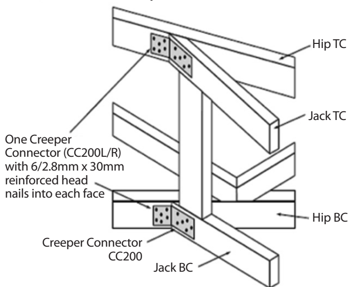
Detail E2 - Jack Truss to Hip Truss (maximum jack station 2400mm)
