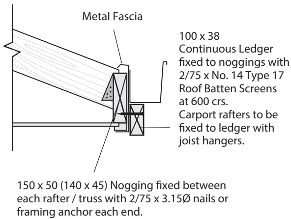
Figure 7 – Strengthening metal fascias to attach pergola rafters
