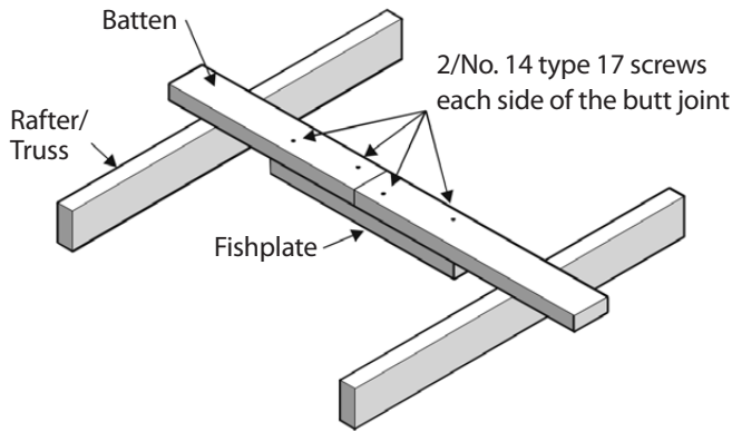
Figure 2 – Joining battens at supports
